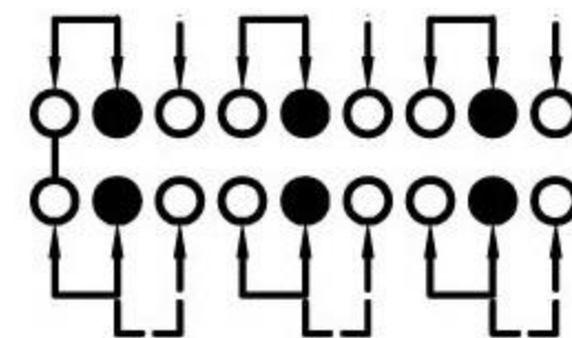
SCHEMATIC (NON-SHORTING)
